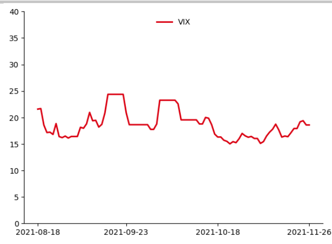
图 6: VIX (%)
